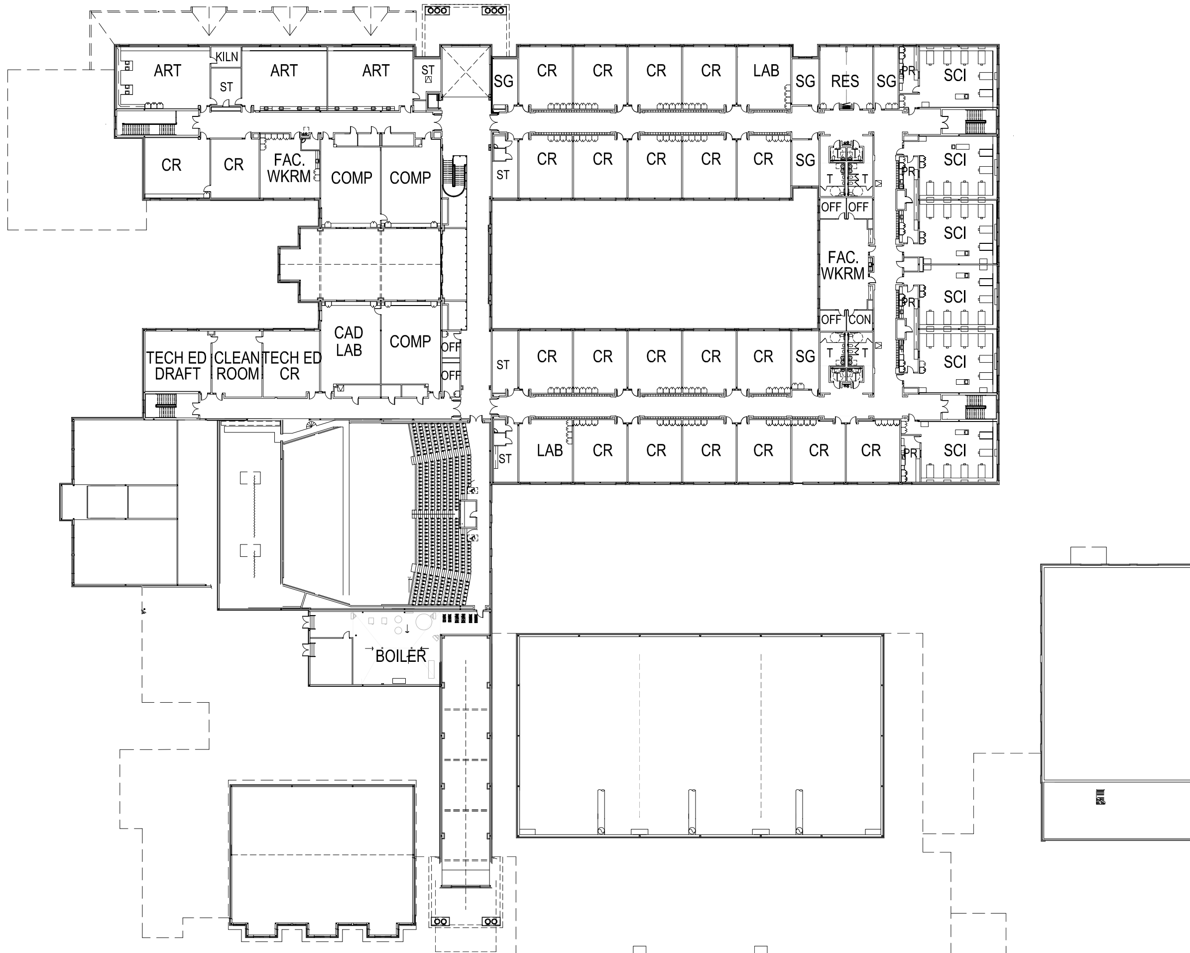
MINNECHAUG REGIONAL HIGH SCHOOL - SECOND FLOOR PLAN
